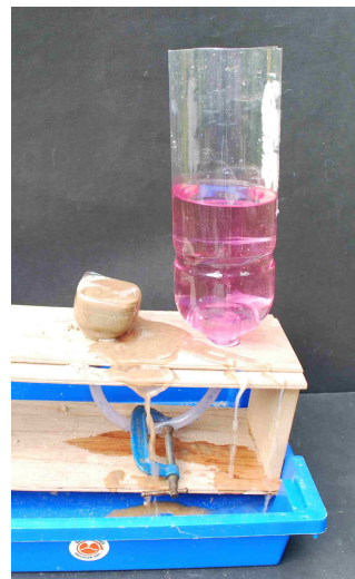
A few seconds later, after the clamp was loosened, the ‘building’ has sunk, as the pore water pressure of the sand increased. ( Photos: Peter Kennett )
