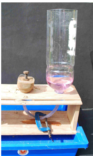
A more elaborate home-made apparatus, ready to close the clamp and fill the right-hand bottle
