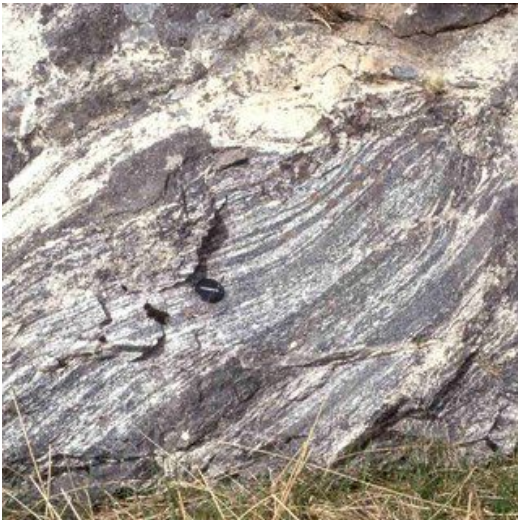
1. Gneiss at outcrop, Isle of Coll, Hebrides, Scotland (lens cap is 50mm diameter)
