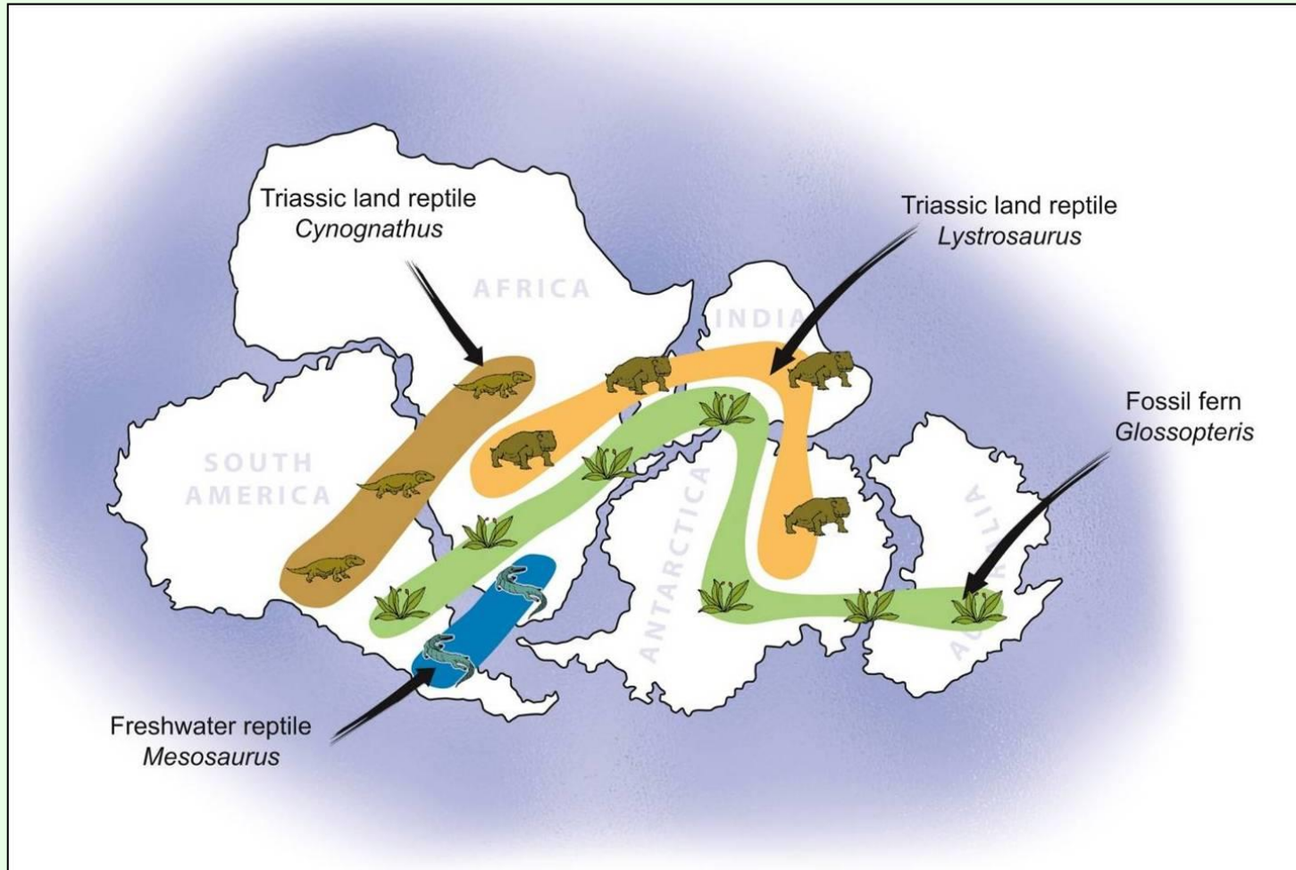
The continental jigsaw puzzles fossil distribution evidence, reproduced with kind permission of USGS
