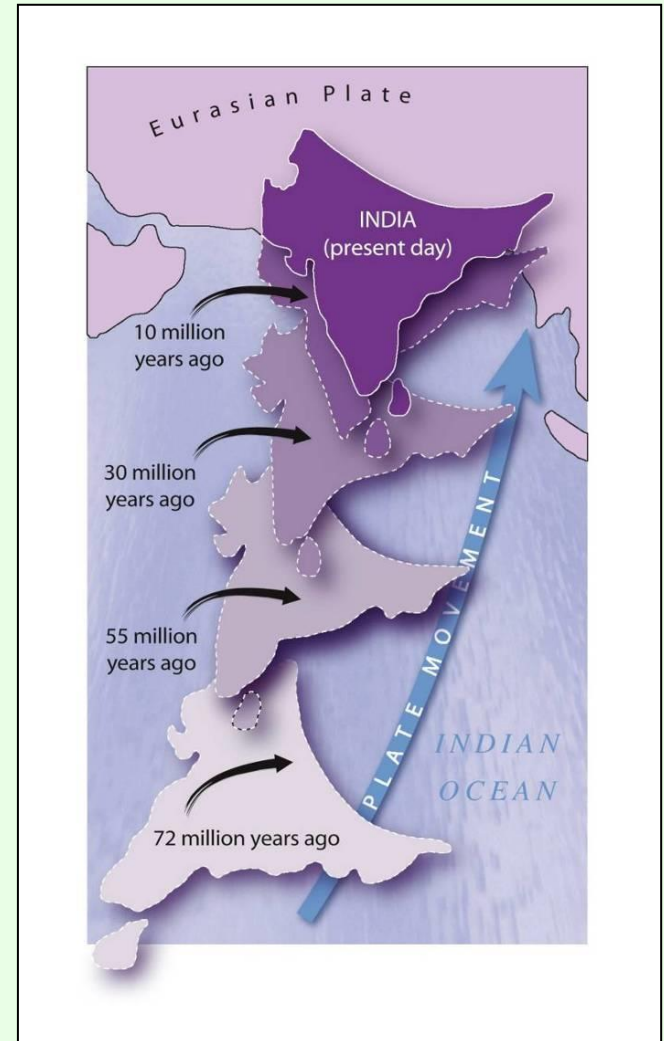
Eurasian Plate (India's movement) © This Dynamic Earth: the Story of Plate Tectonics, USGS, redrawn by ESEU
