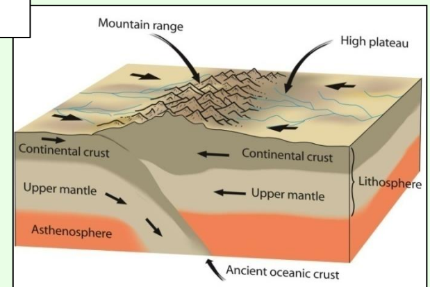
Continental plate collision zone. Reproduced with kind permission of USGS, redrawn by ESEU
