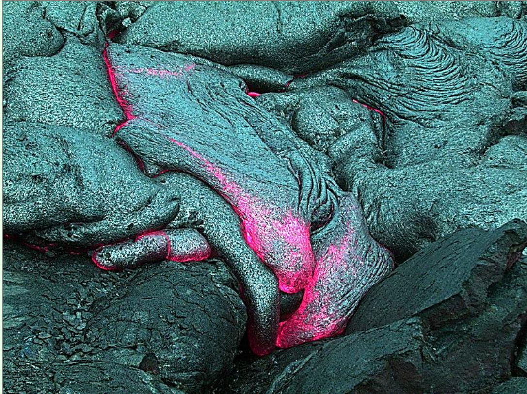
Underwater basalt lava at a divergent margin in the public domain by Vintei
