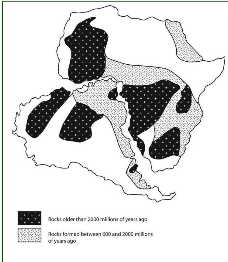
The distribution of ancient rocks across South America and Africa © Andrew McLeish in 'Geological Science'
