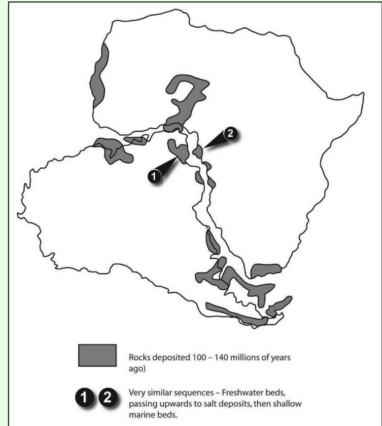
The distribution of younger rocks across South America and Africa up to the beginning of the continental split. Source unknown, redrawn by ESEU
