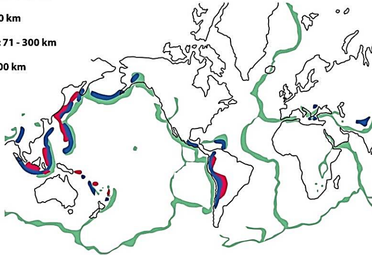
Distribution of earthquakes – source unknown, redrawn by ESEU
