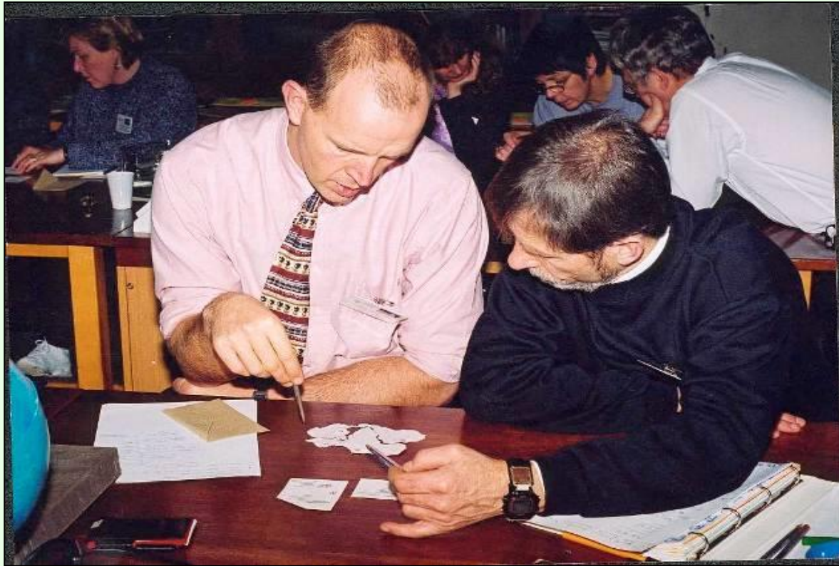
Debating the reconstruction of the supercontinent of 'Gondwana' © Peter Kennett
