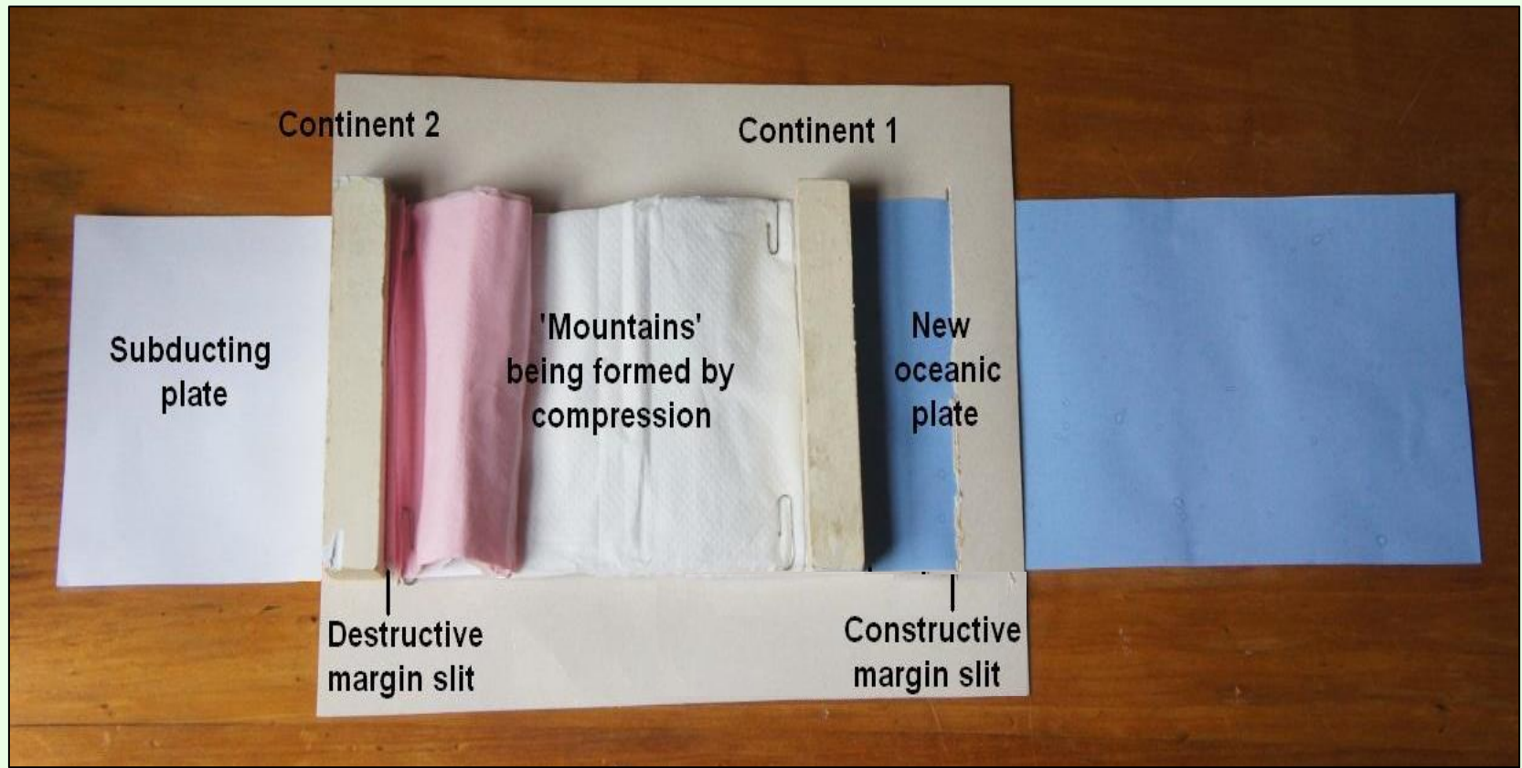
Photograph of plates in motion © Chris King
