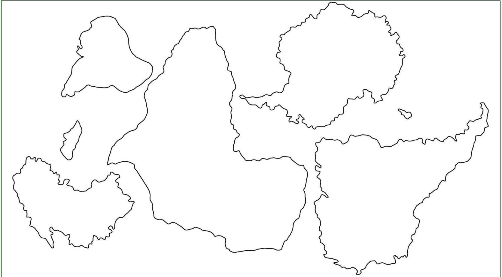
The continental jigsaw puzzle (the outlines of the Gondwana continents) © Author/origin unknown – redraw by Peter Kennett
