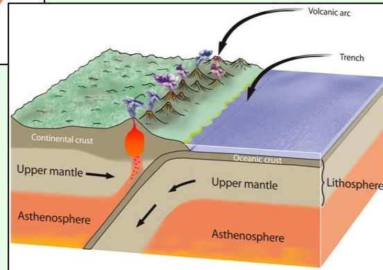
Subduction zone ('partially melts and volcanoes are produced' 'molten rock cools down below the surface') - reproduced with kind permission of USGS, redrawn by ESEU
