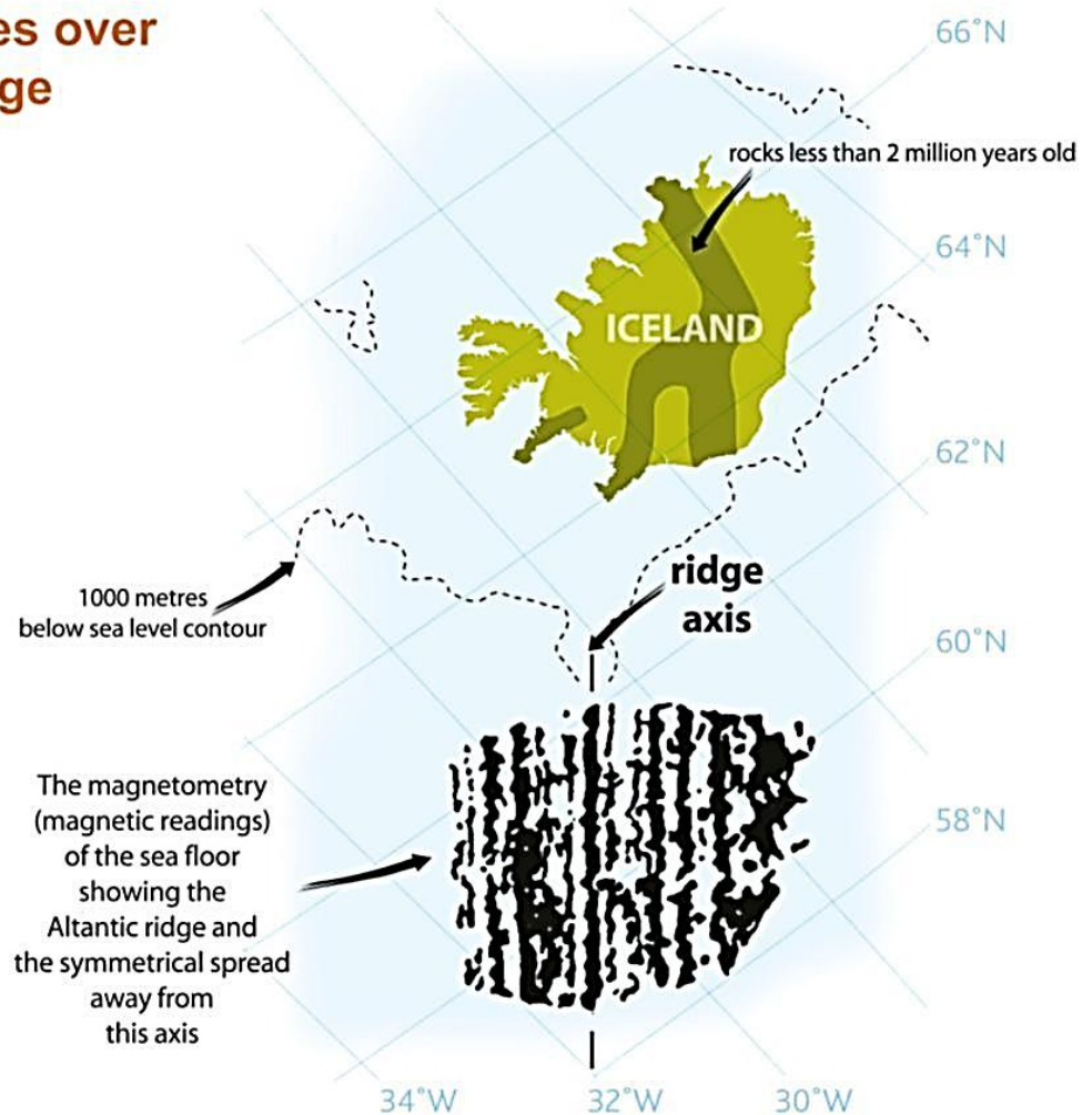
Magnetic anomalies over the Reykjanes Ridge © Geoscience, redrawn by ESEU
